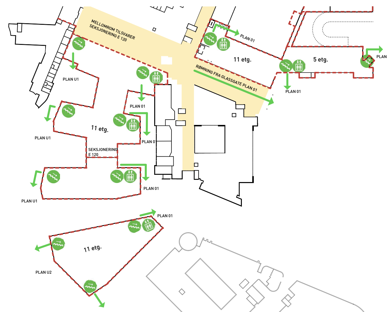
Figur 8.6 Prinsippbrannplan, rømning, brannheiser.
